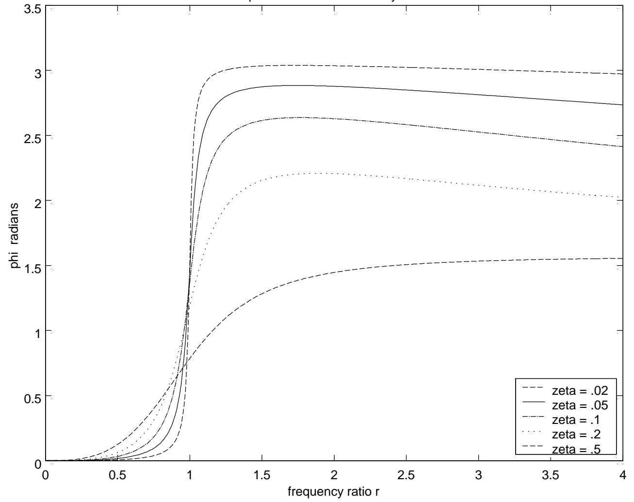
Displacement Transmissibility Phase
