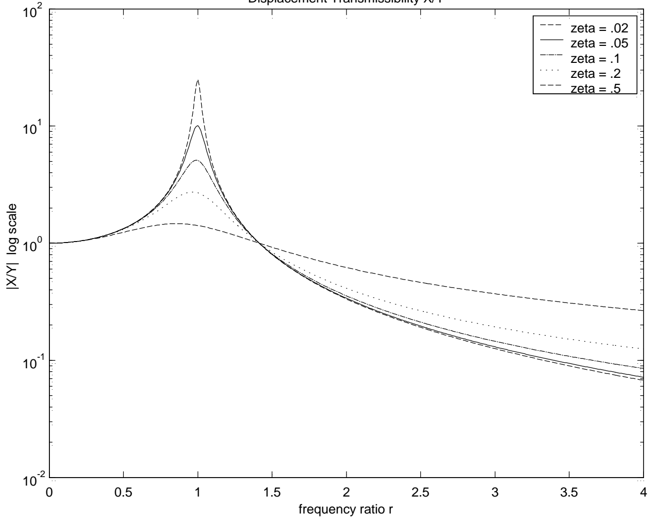
Displacement Transmissibility X/Y
