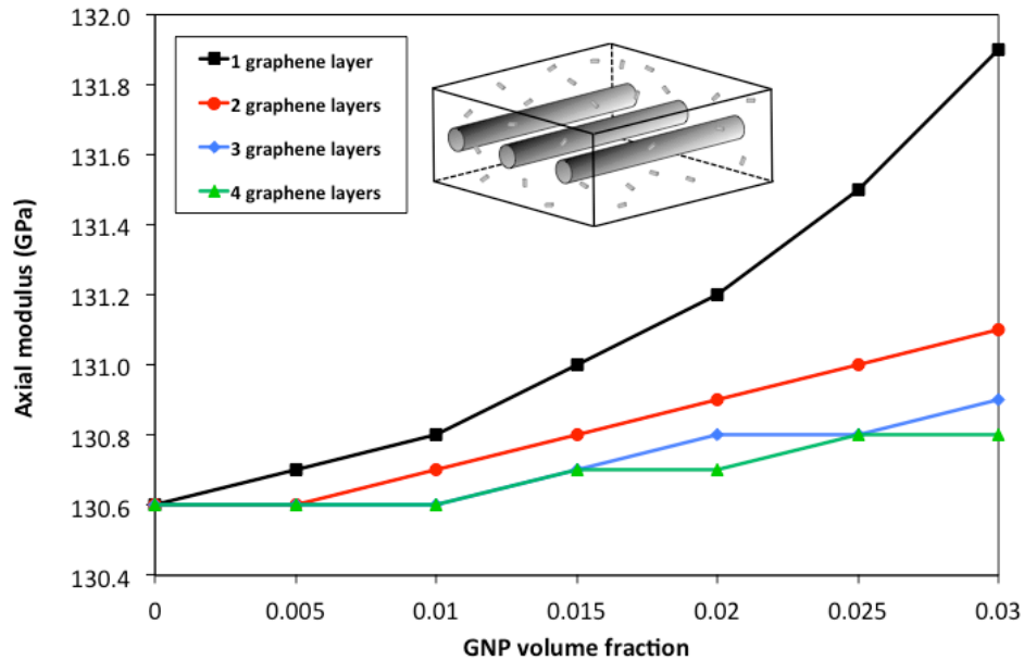
Fig. 12 Predicted axial modulus for GNP/carbon fiber/epoxy hybrid composite for varying GNP volume fraction and GNP layers.
