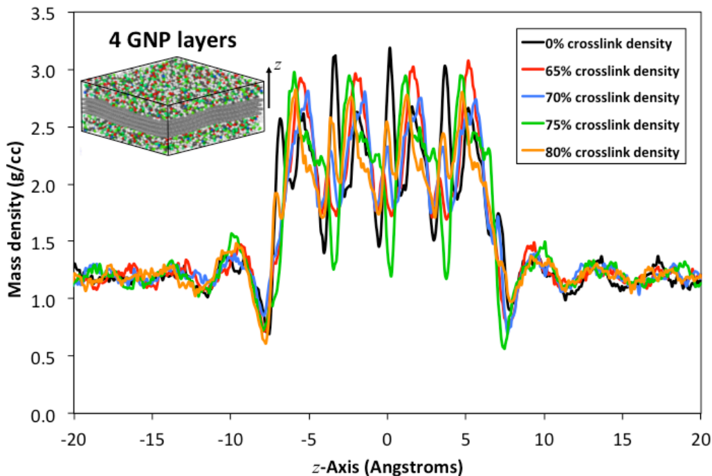
Fig. 8 Atomic mass density profile along z-axis for 4 layers of graphene
