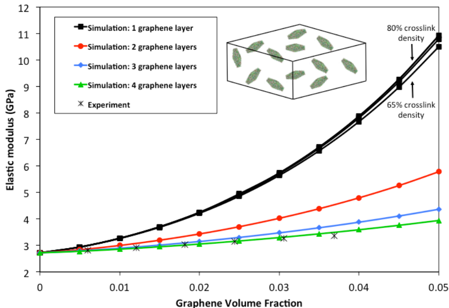
Fig. 15 Elastic modulus of GNP/epoxy composite for both computational and experimental approaches.
