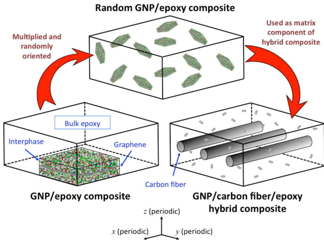
Fig. 10 Multiscale modeling scheme
