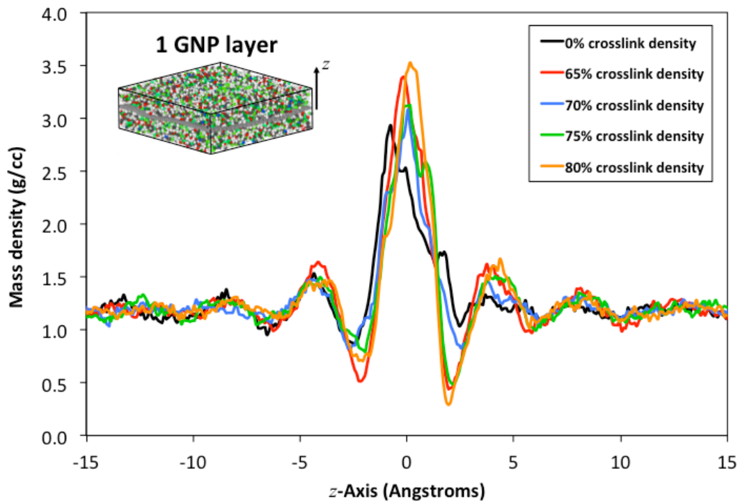
Fig. 5 Atomic mass density profile along z -axis for 1 layer of graphene
