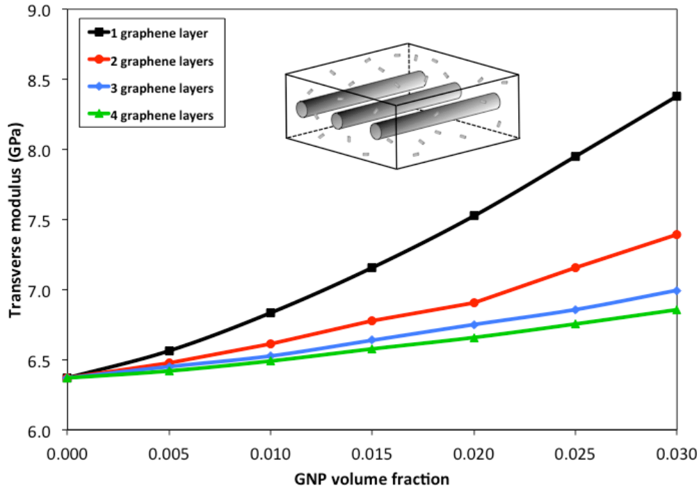
Fig. 13 Predicted transverse modulus for GNP/carbon fiber/epoxy hybrid composite for varying GNP volume fractions and GNP layers.
