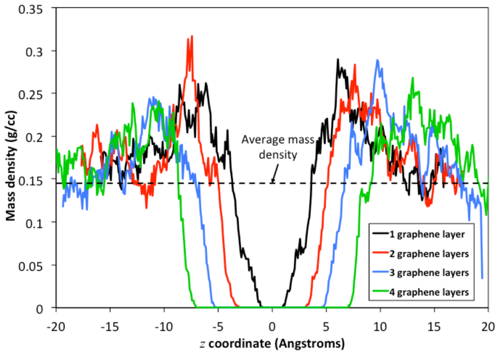
Fig. 4. Mass density profile of crosslinked atoms as a function of z -axis coordinate for 80% crosslinked systems. The center of the MD model corresponds to z = 0 .
