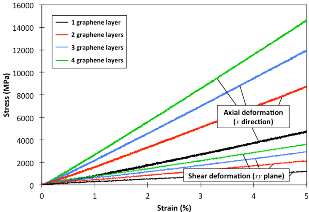
Fig. 9. Representative axial and shear Stress vs. strain curves for 80% crosslinked structures
