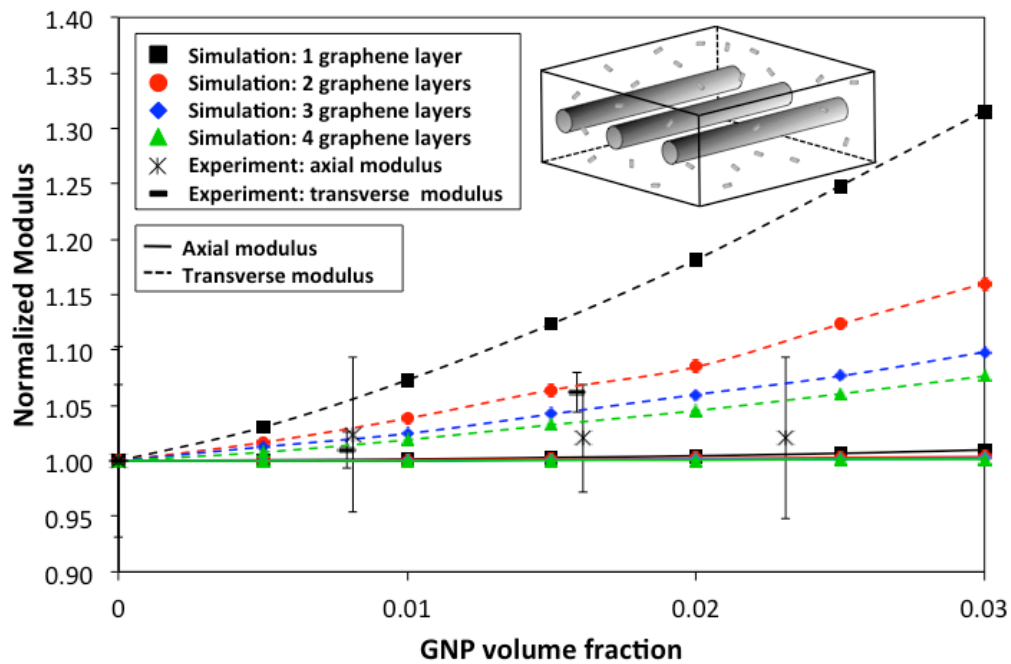
Fig. 16 Normalized axial and transverse modulus of GNP/carbon fiber/epoxy composite for both computational and experimental approaches.
