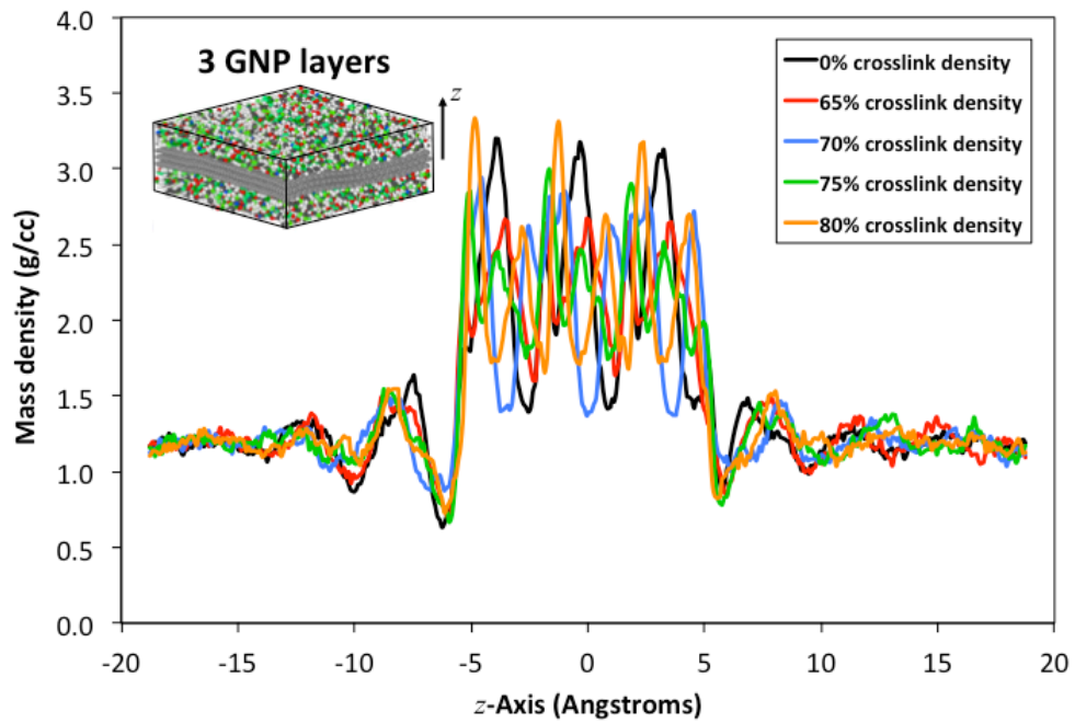
Fig. 7 Atomic mass density profile along z -axis for 3 layers of graphene
