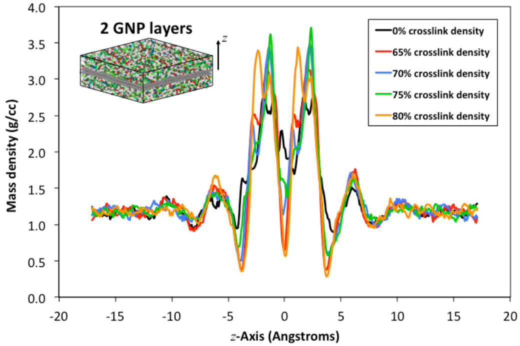
Fig. 6 Atomic mass density profile along z -axis for 2 layers of graphene
