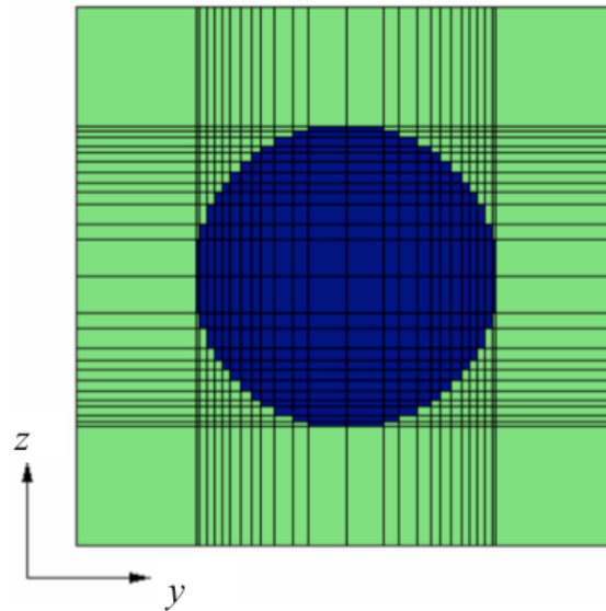
Fig. 11 MAC/GMC repeat unit cell for the GNP/carbon fiber/epoxy hybrid composite (ARCHID=13)
