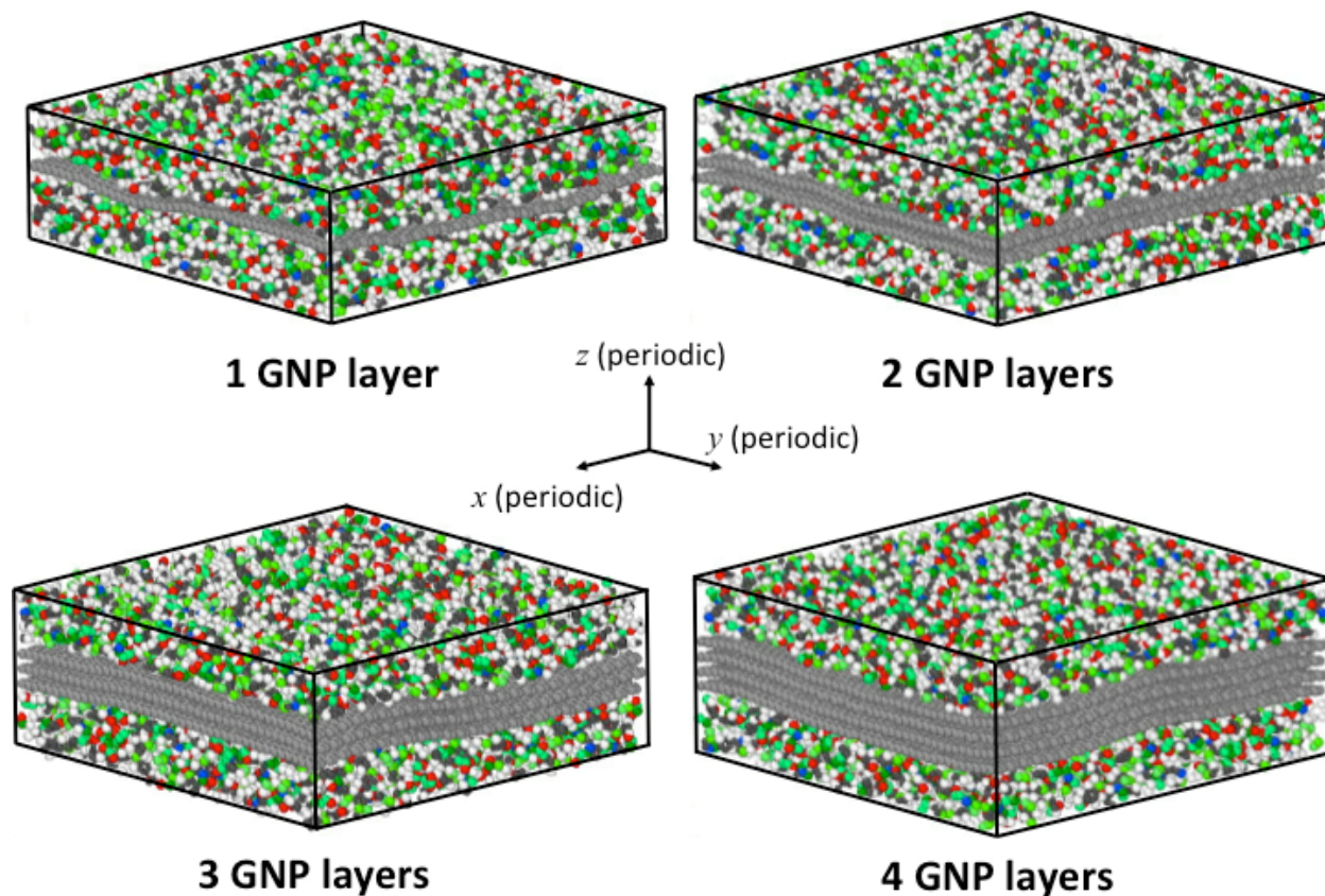
Fig. 3. Equilibrated models for varying number of graphene layers before crosslinking. Average polymer density \sim 1.17 g/cc for each model.
