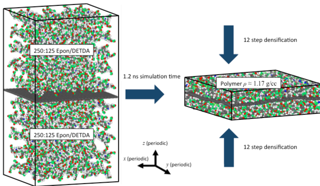
Fig. 2. Molecular structures for single graphene sheet system highlighting the densification process. Gray atoms - carbon; white atoms - hydrogen; red atoms - oxygen; blue atoms - nitrogen; green atoms - united atoms ( CH , CH_2 , CH_3 )
